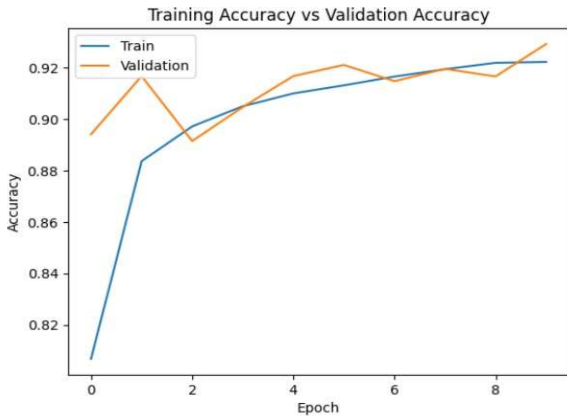
Fig 4.1: Graph between Training Accuracy and Validation Accuracy
