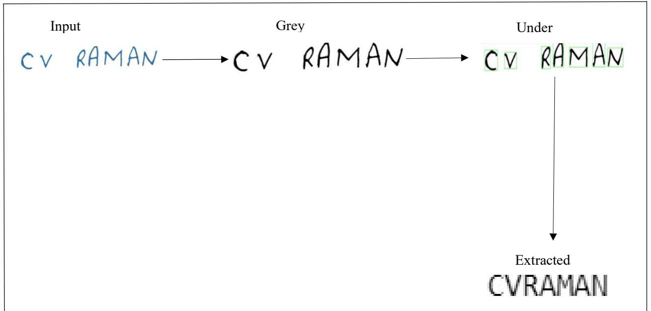
Fig 3.3: Flow Chart of the model with an example
